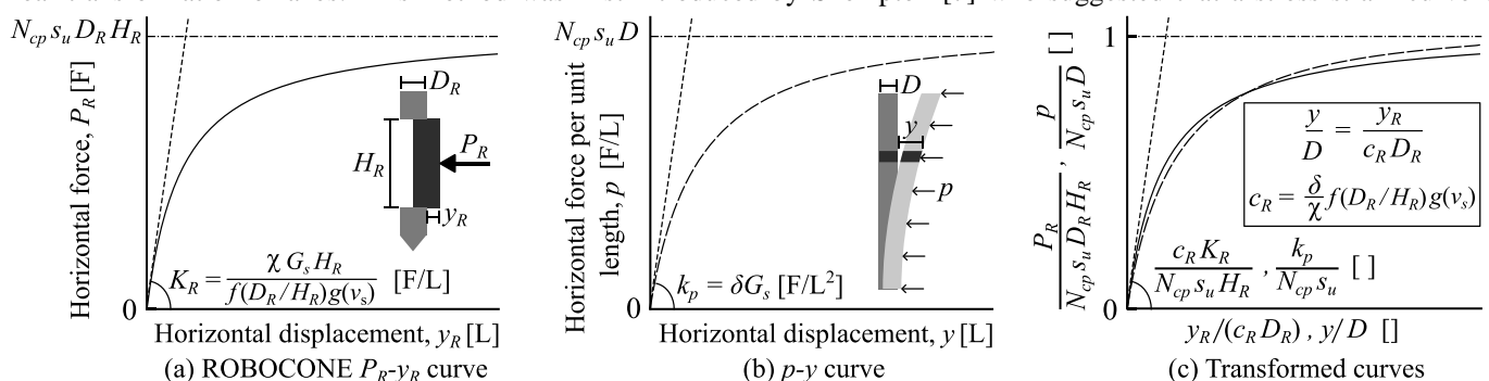
Figure 1: Illustration of the similarity concept applied to relate a ROBOCONE P_R - y_R curve to a p - y curve in clay.
