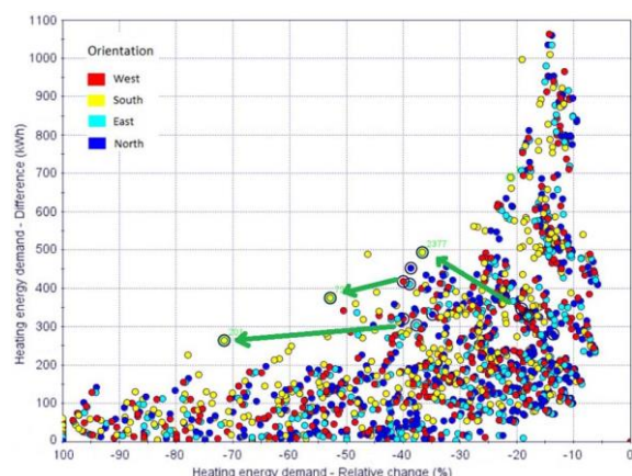
Fig. 8a – Difference in heating demand (absolute and relative) between room without and with Trombe wall for different orientations [13]. Positive absolute values / negative percentages denote that the Trombe wall leads to an energy saving. The green arrows denote how certain cases change if their orientation changes.
