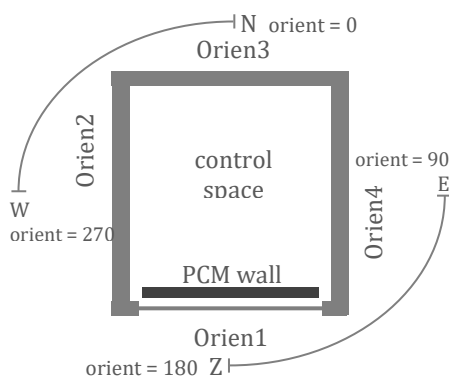
Fig. 4 – Floor plan model of the simulated room. The orientation may vary in the model.
