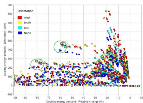
Fig. 8b – Difference in cooling demand (absolute and relative) between room without and with Trombe wall for different orientations [13]. Positive absolute values / negative percentages denote that the Trombe wall leads to an energy saving. The green circles denote how certain cases change if their orientation changes.
