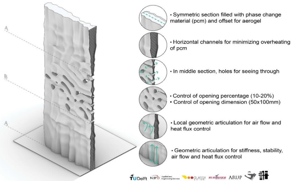
Fig. 14 – Final design of the prototype of the Double Face 2.0 PCM-based rotatable Trombe wall.
